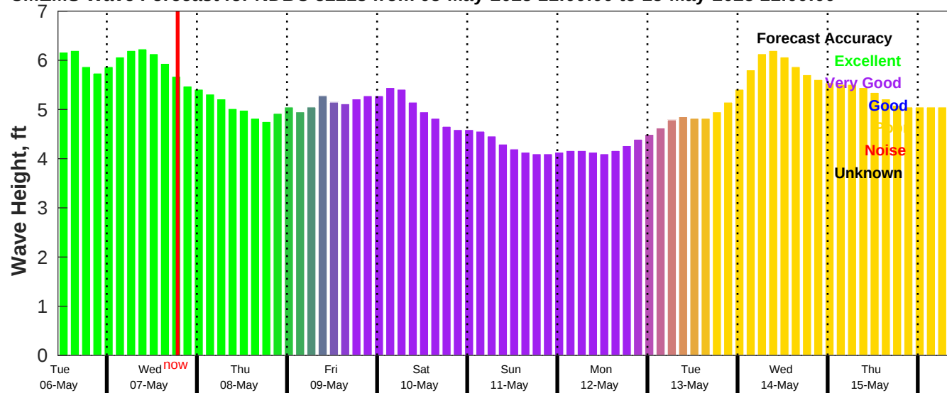
CEEMS Wave Forecast for NDBC 52213 from 05-May-2025 11:00:00 to 15-May-2025 11:00:00
