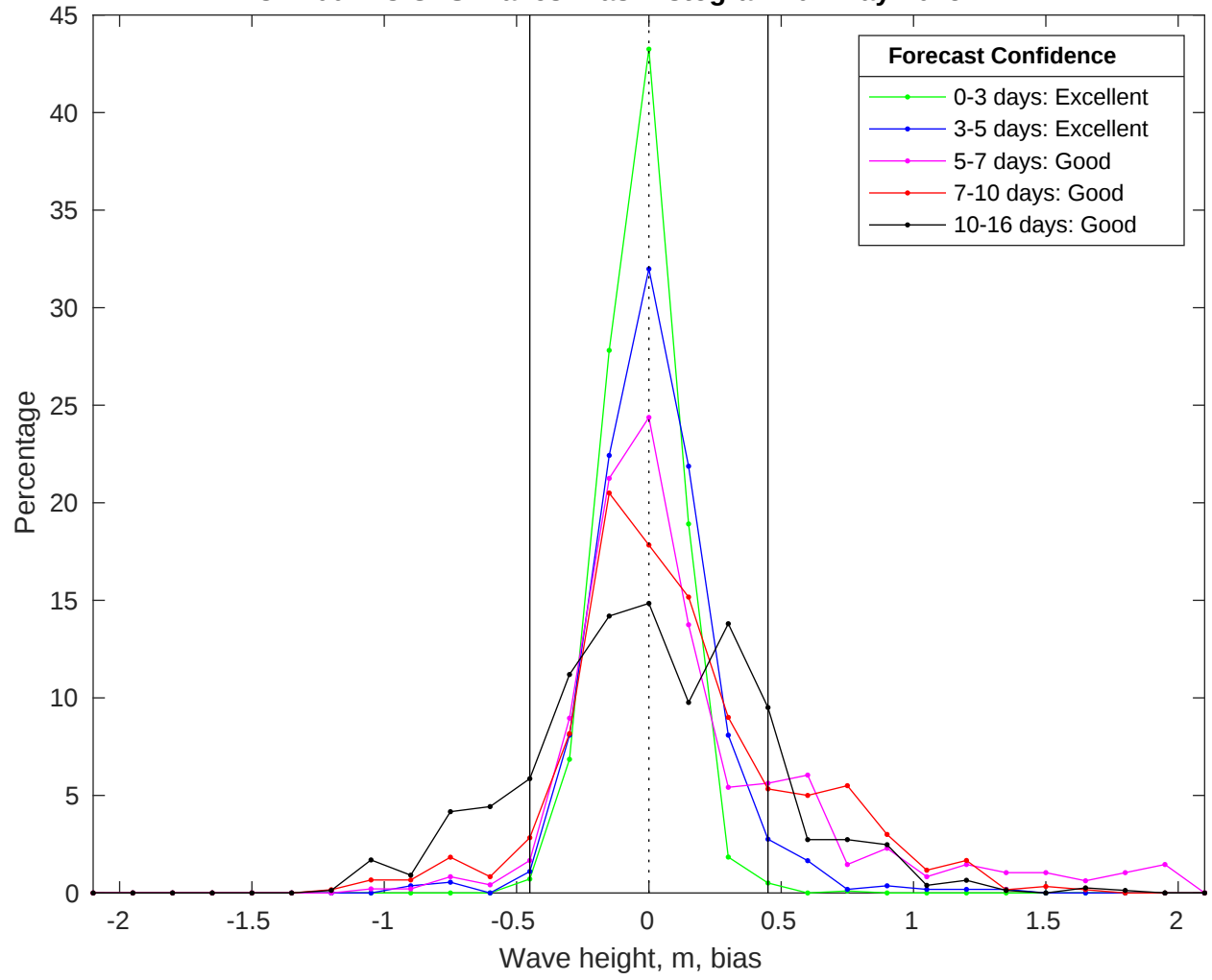
NDBC 41004 vs GFS Waves Bias Histogram: 07-May-2025
