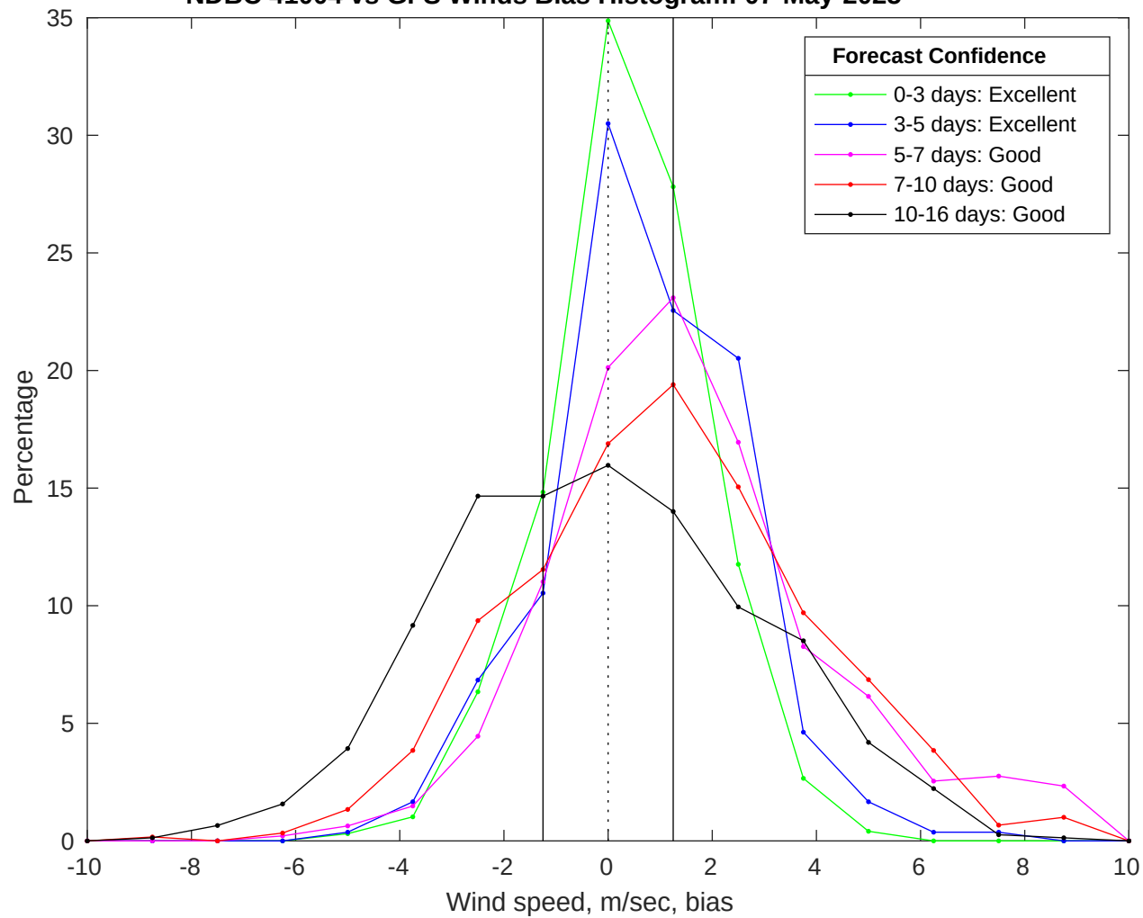
NDBC 41004 vs GFS Winds Bias Histogram: 07-May-2025
