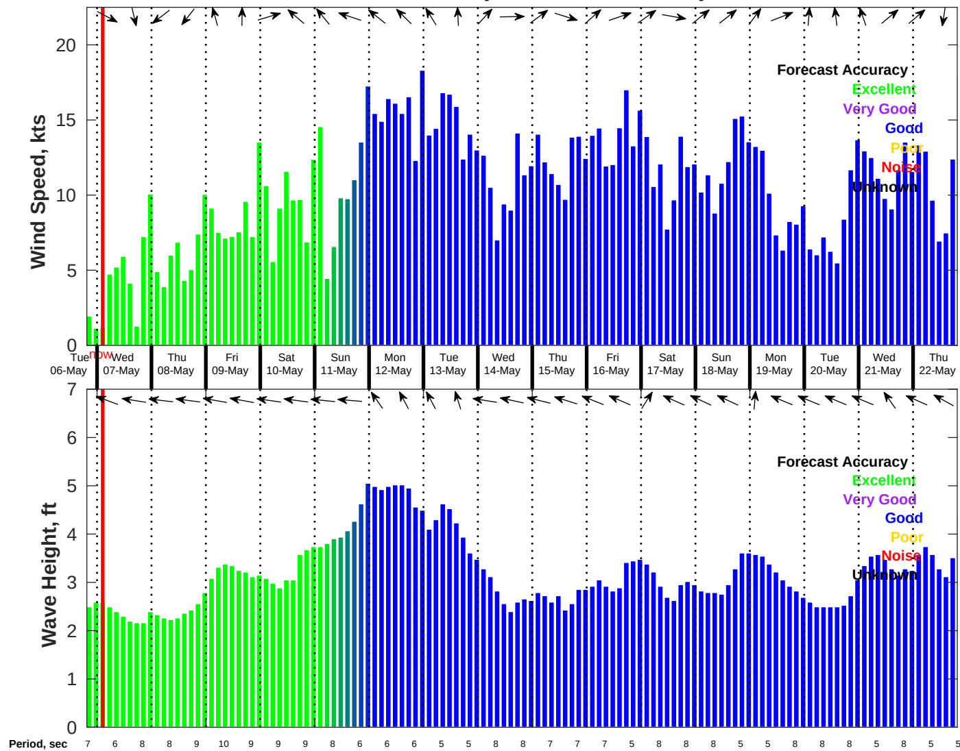
Wind & Wave Forecast for NDBC 41004 from 06-May-2025 19:00:00 to 22-May-2025 19:00:00
