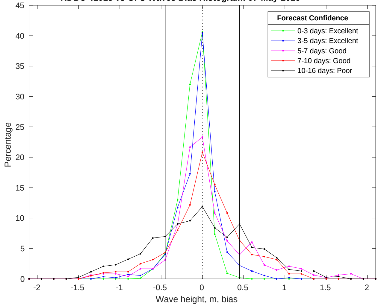
NDBC 41013 vs GFS Waves Bias Histogram: 07-May-2025
