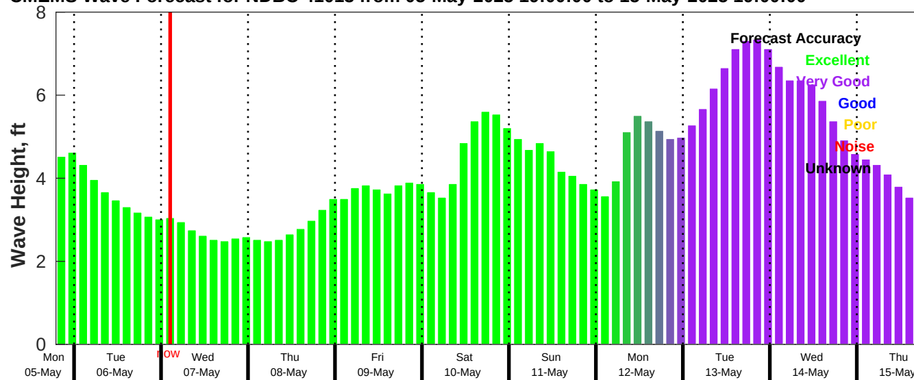
CMEMS Wave Forecast for NDBC 41013 from 05-May-2025 19:00:00 to 15-May-2025 19:00:00
