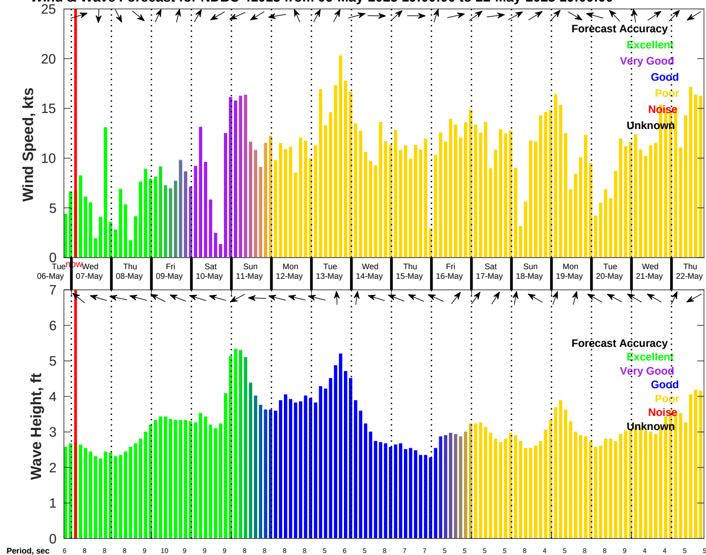
Wind & Wave Forecast for NDBC 41013 from 06-May-2025 19:00:00 to 22-May-2025 19:00:00
