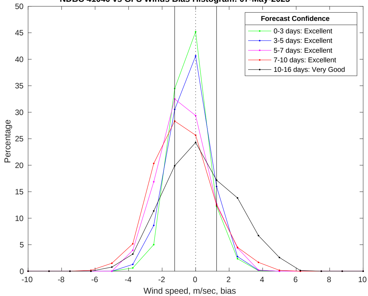
NDBC 41040 vs GFS Winds Bias Histogram: 07-May-2025
