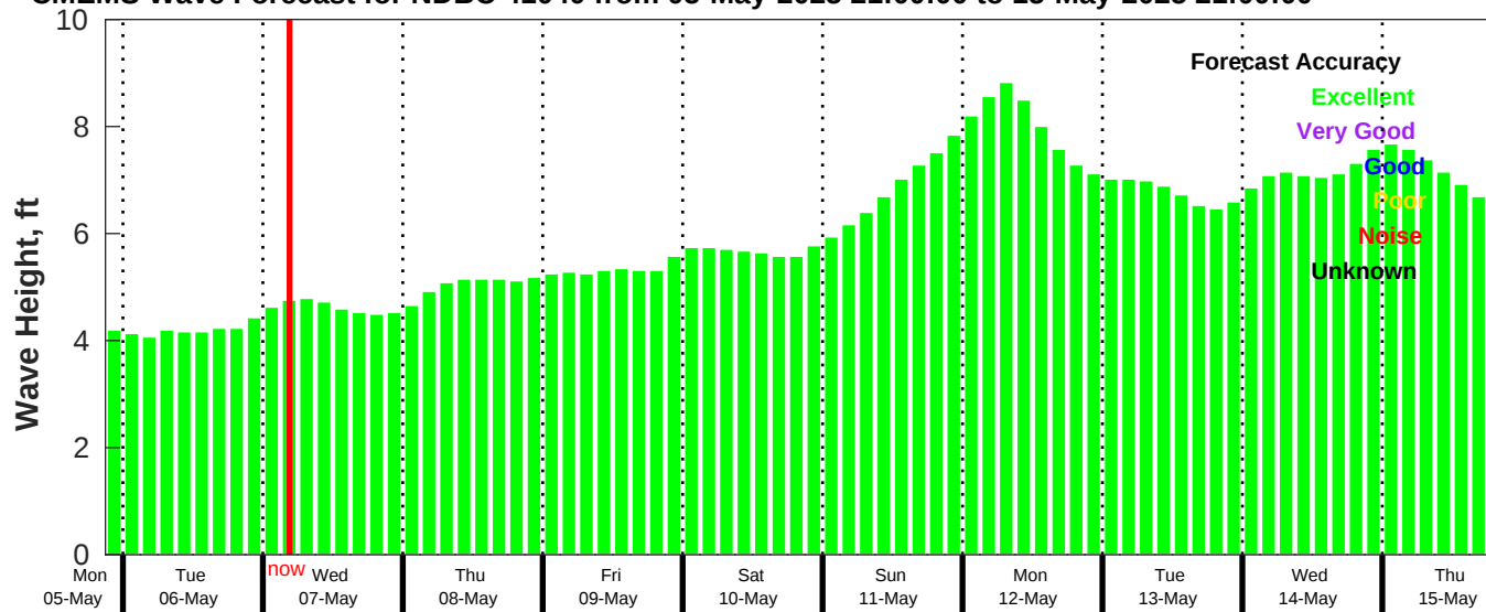
CMEMS Wave Forecast for NDBC 41040 from 05-May-2025 21:00:00 to 15-May-2025 21:00:00
