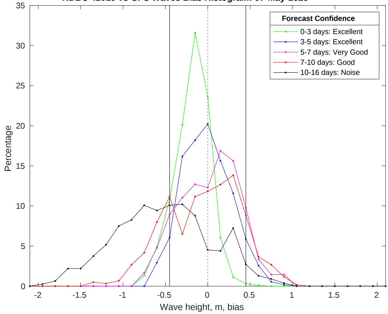
NDBC 42019 vs GFS Waves Bias Histogram: 07-May-2025
