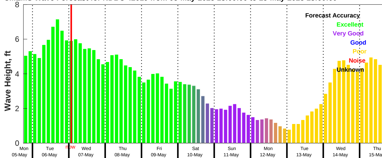
CMEMS Wave Forecast for NDBC 42019 from 05-May-2025 18:00:00 to 15-May-2025 18:00:00
