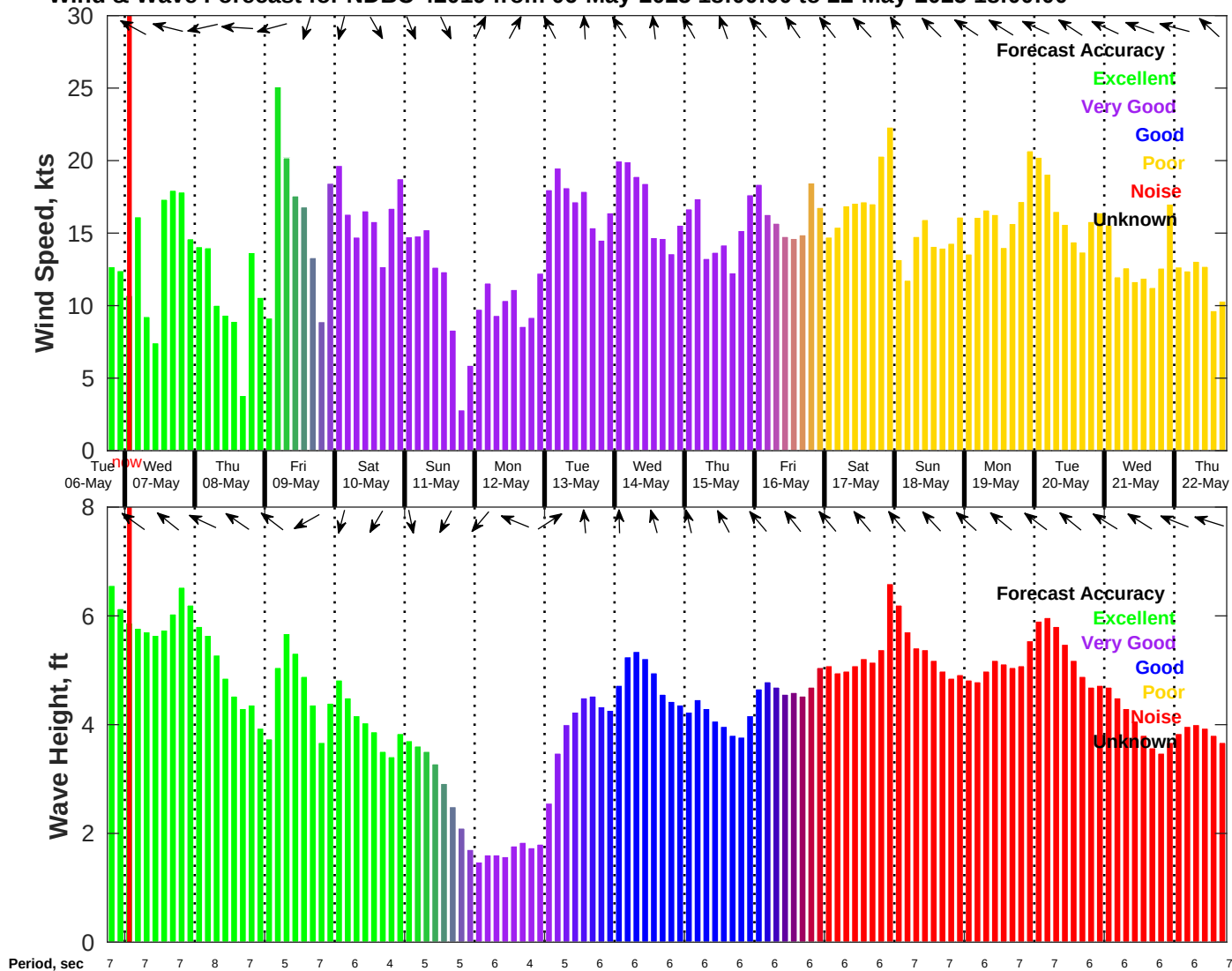
Wind & Wave Forecast for NDBC 42019 from 06-May-2025 18:00:00 to 22-May-2025 18:00:00
