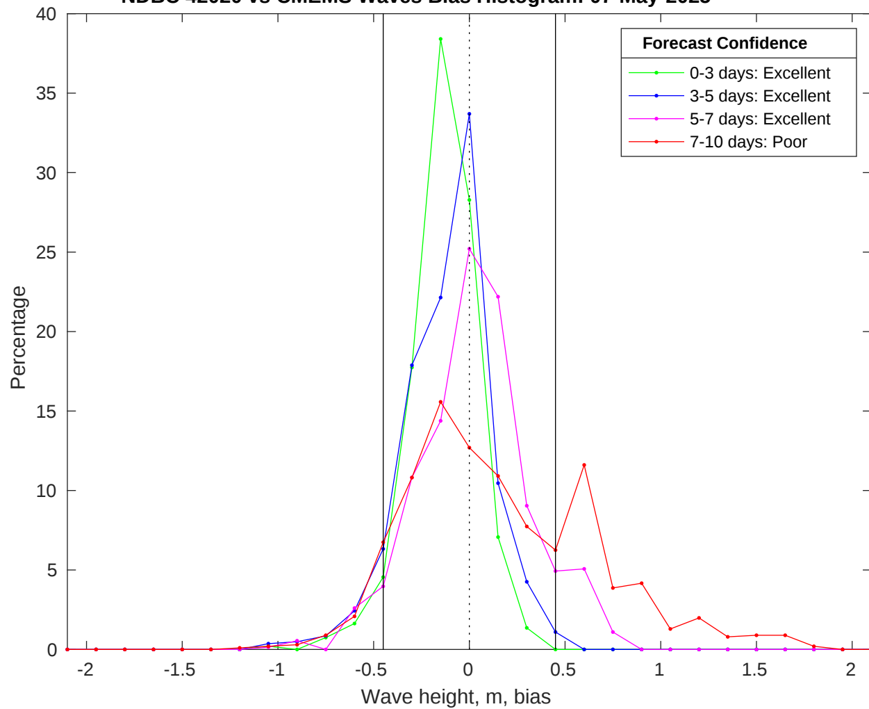
NDBC 42020 vs CMEMS Waves Bias Histogram: 07-May-2025
