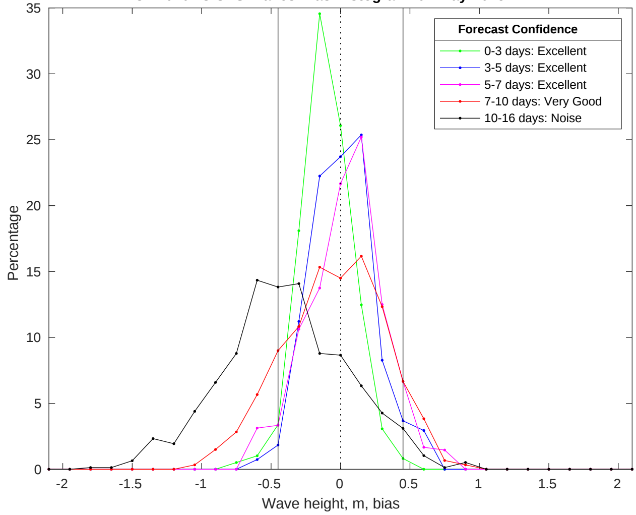
NDBC 42020 vs GFS Waves Bias Histogram: 07-May-2025
