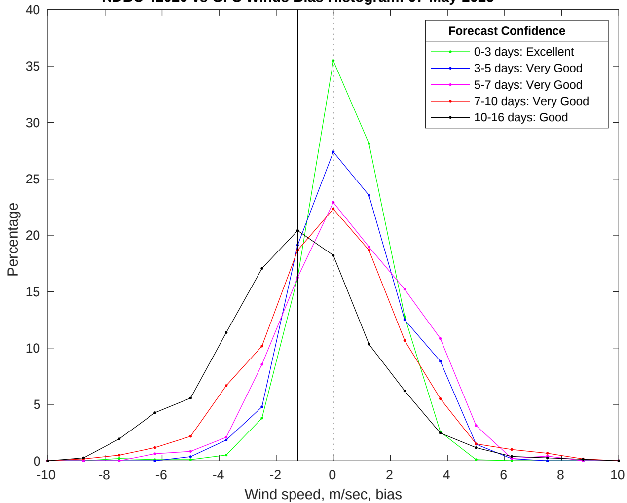
NDBC 42020 vs GFS Winds Bias Histogram: 07-May-2025
