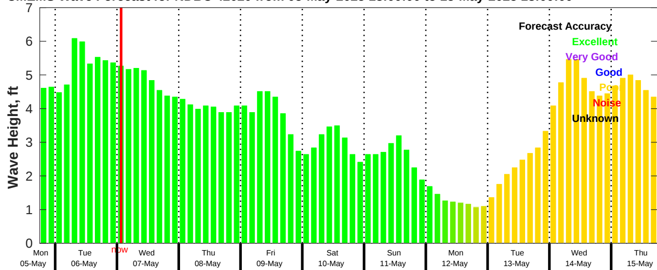
CMEMS Wave Forecast for NDBC 42020 from 05-May-2025 18:00:00 to 15-May-2025 18:00:00
