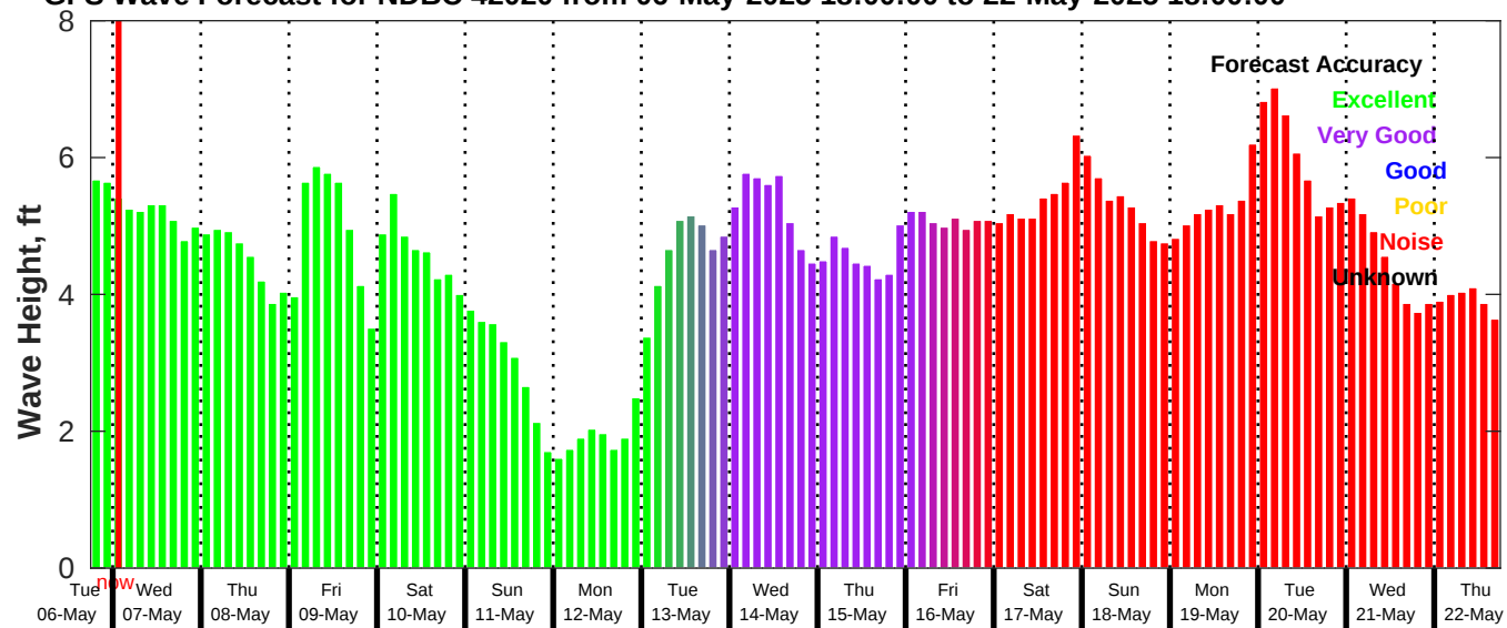
GFS Wave Forecast for NDBC 42020 from 06-May-2025 18:00:00 to 22-May-2025 18:00:00
