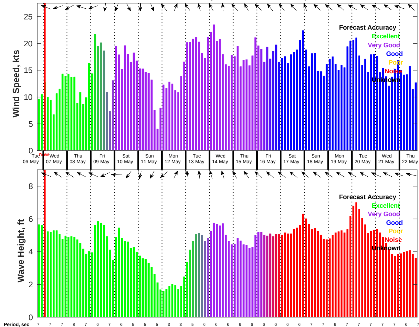
Wind & Wave Forecast for NDBC 42020 from 06-May-2025 18:00:00 to 22-May-2025 18:00:00
