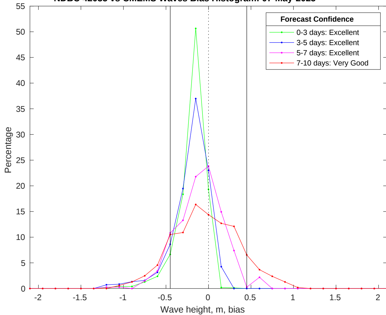
NDBC 42035 vs CMEMS Waves Bias Histogram: 07-May-2025
