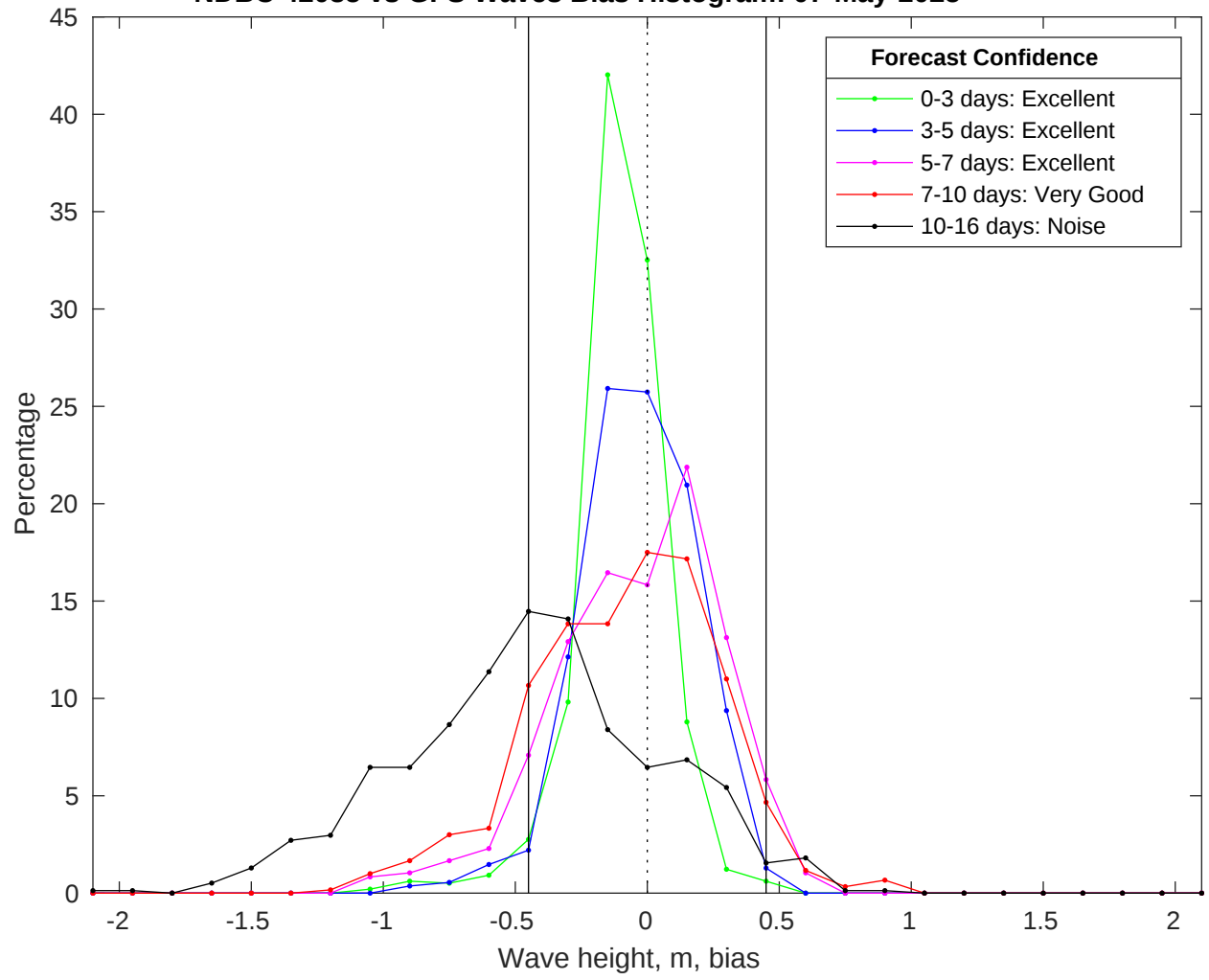
NDBC 42035 vs GFS Waves Bias Histogram: 07-May-2025
