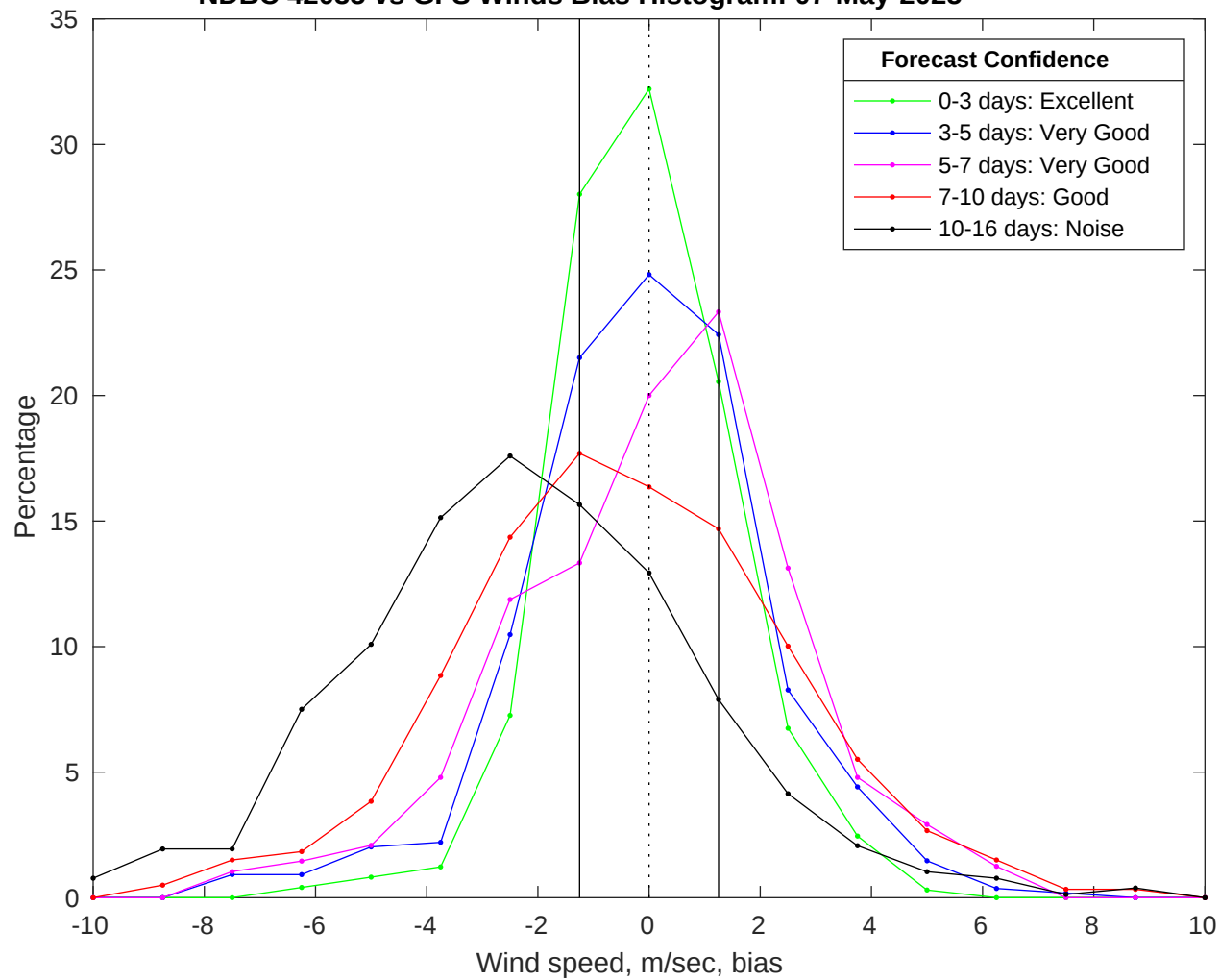
NDBC 42035 vs GFS Winds Bias Histogram: 07-May-2025
