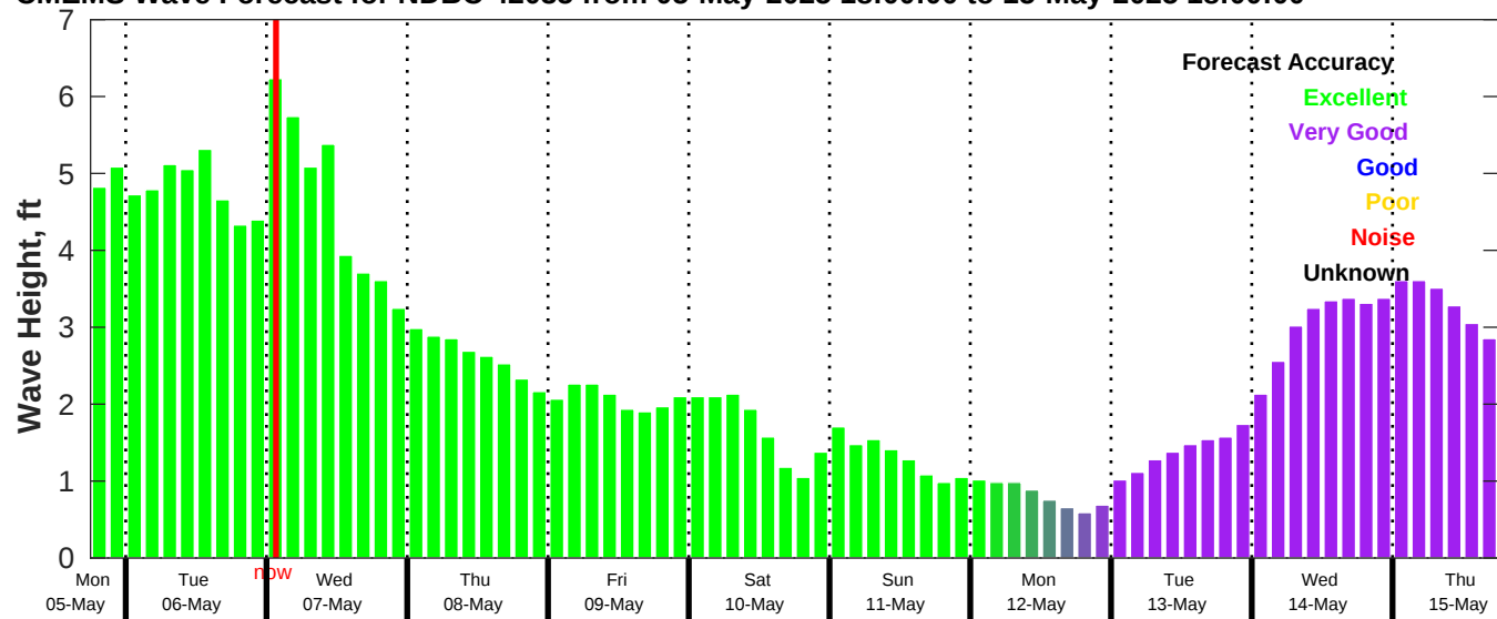
CMEMS Wave Forecast for NDBC 42035 from 05-May-2025 18:00:00 to 15-May-2025 18:00:00
