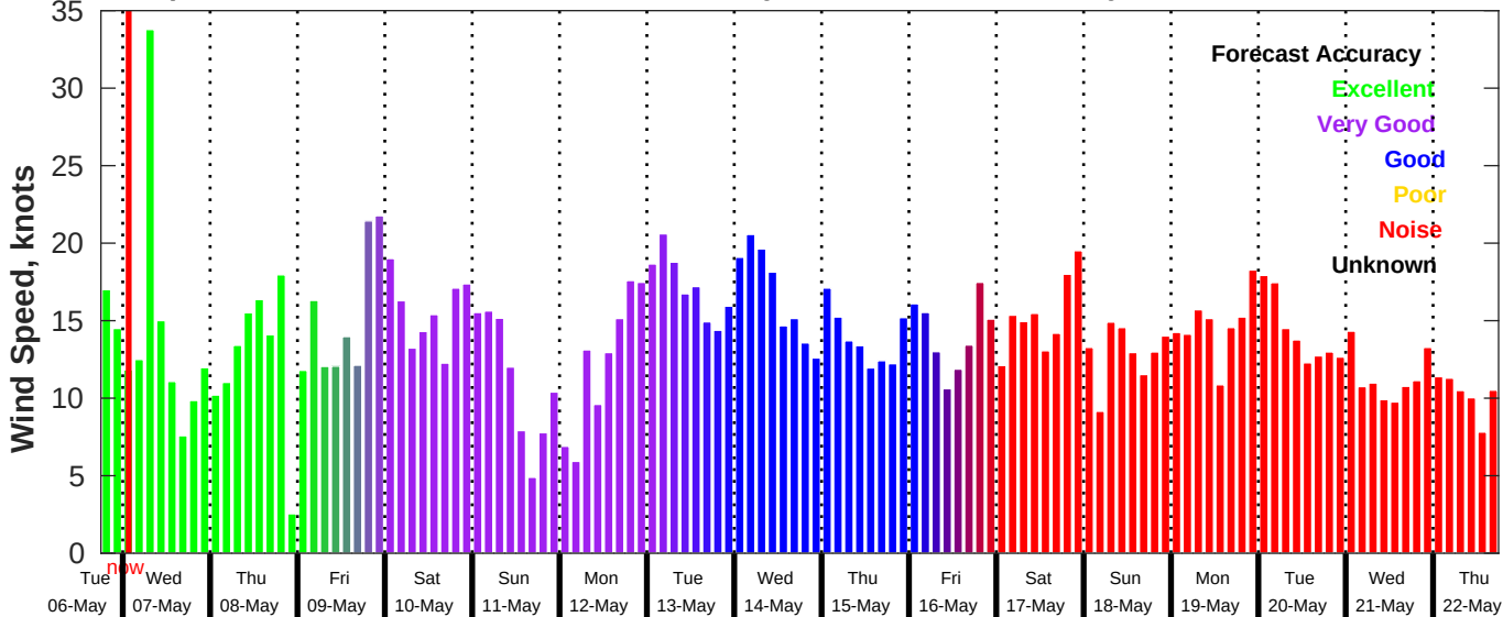
GFS Wind Speed Forecast for NDBC 42035 from 06-May-2025 18:00:00 to 22-May-2025 18:00:00
