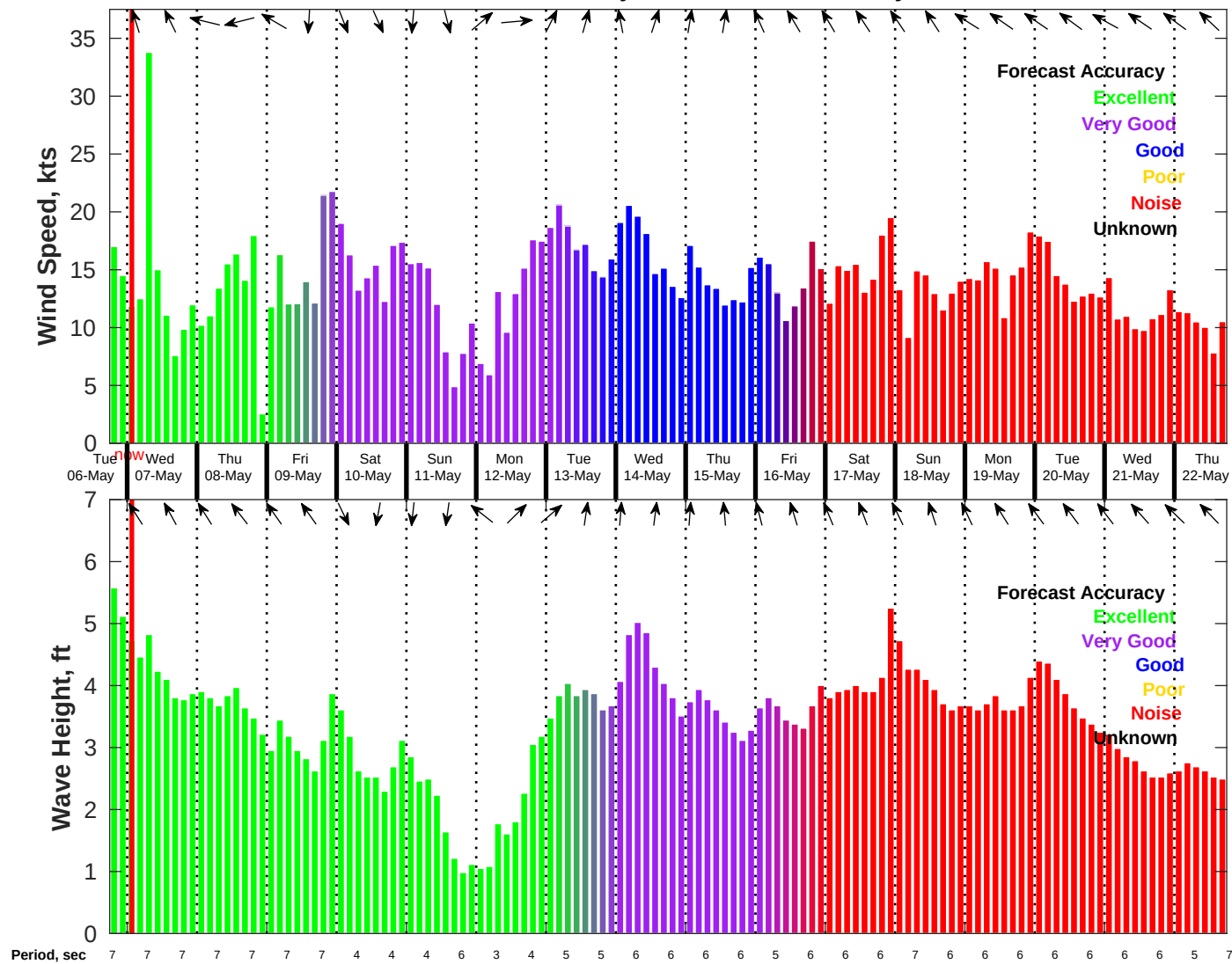
Wind & Wave Forecast for NDBC 42035 from 06-May-2025 18:00:00 to 22-May-2025 18:00:00
