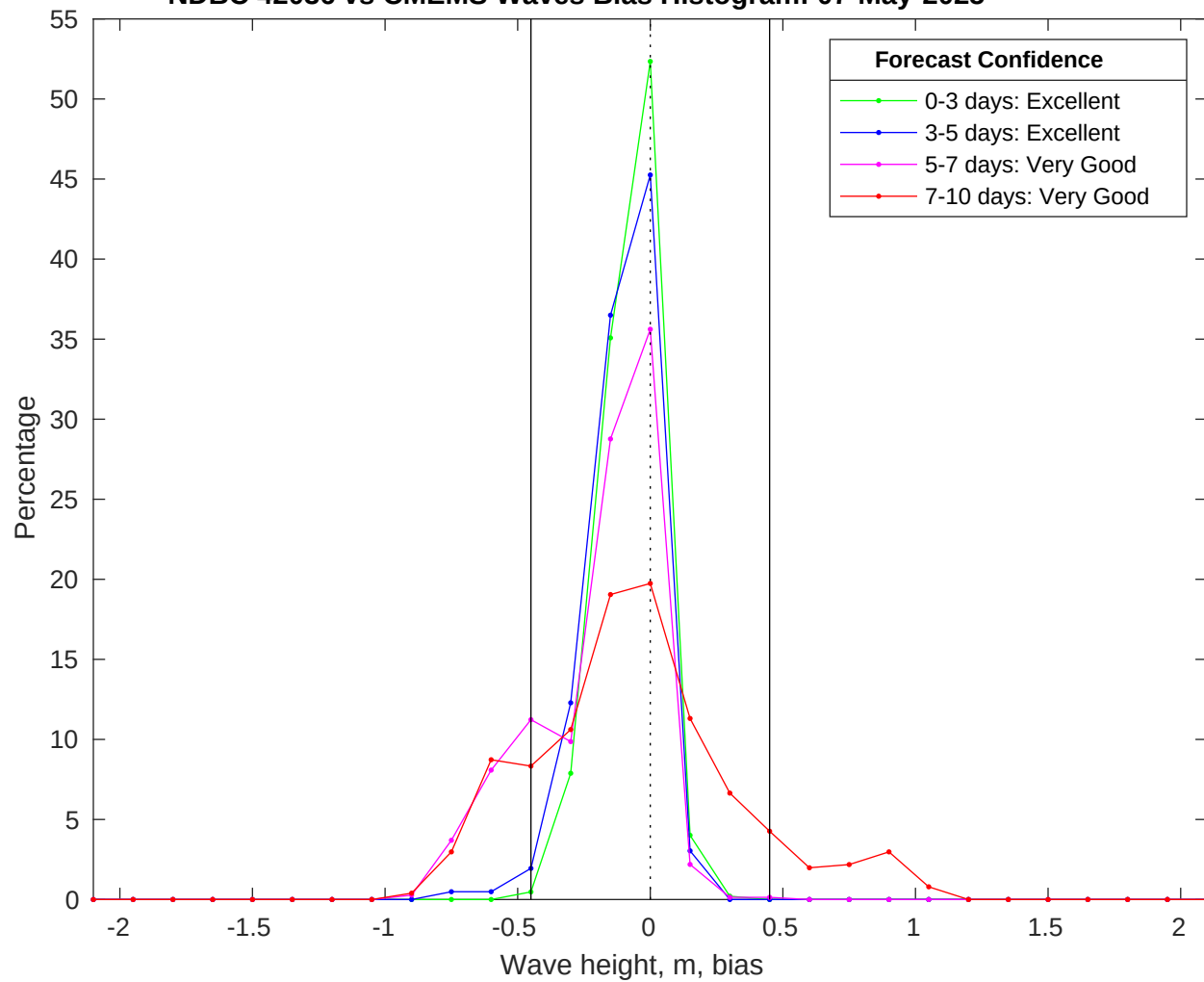
NDBC 42036 vs CMEMS Waves Bias Histogram: 07-May-2025
