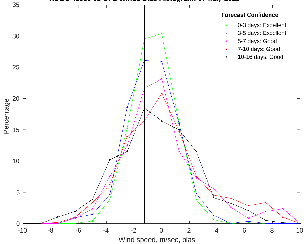
NDBC 42036 vs GFS Winds Bias Histogram: 07-May-2025
