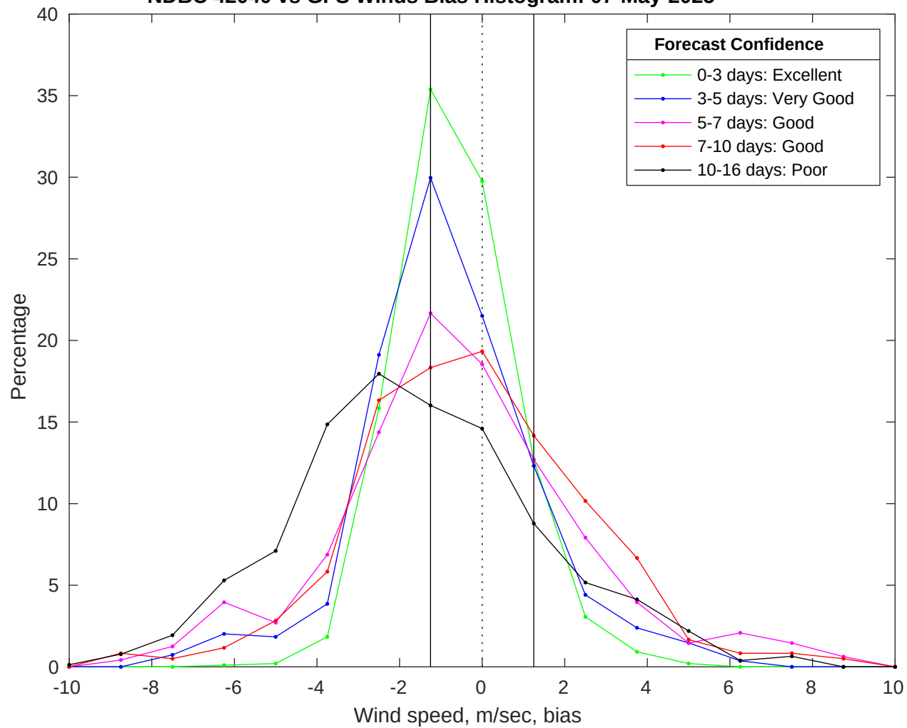
NDBC 42040 vs GFS Winds Bias Histogram: 07-May-2025
