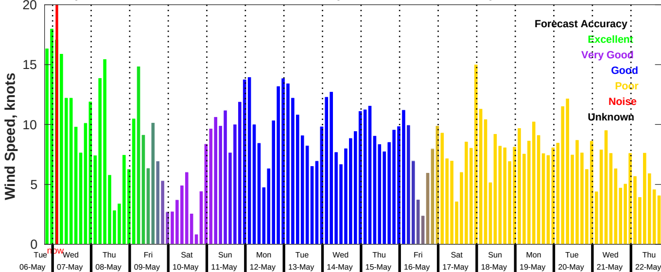
GFS Wind Speed Forecast for NDBC 42040 from 06-May-2025 19:00:00 to 22-May-2025 19:00:00
