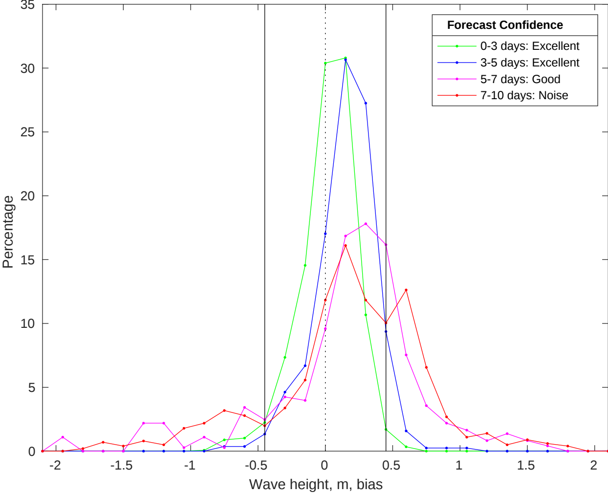
NDBC 46011 vs CMEMS Waves Bias Histogram: 07-May-2025
