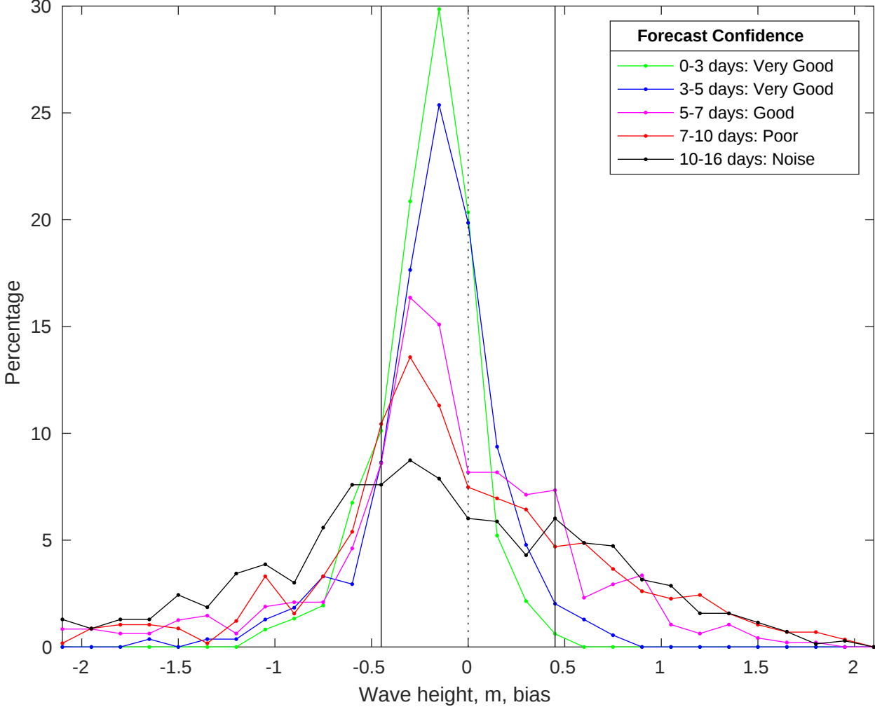
NDBC 46011 vs GFS Waves Bias Histogram: 07-May-2025
