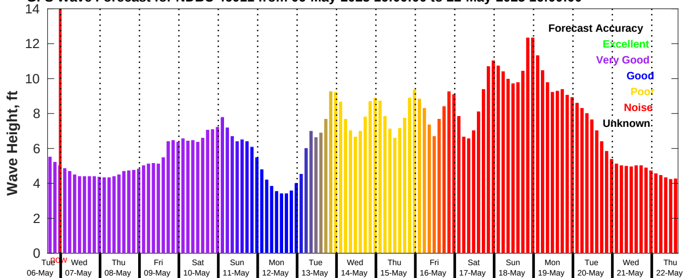
GFS Wave Forecast for NDBC 46011 from 06-May-2025 16:00:00 to 22-May-2025 16:00:00
