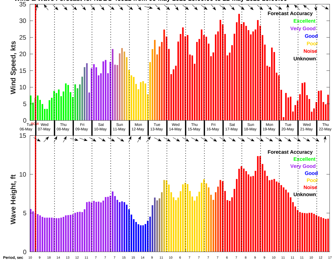
Wind & Wave Forecast for NDBC 46011 from 06-May-2025 16:00:00 to 22-May-2025 16:00:00
