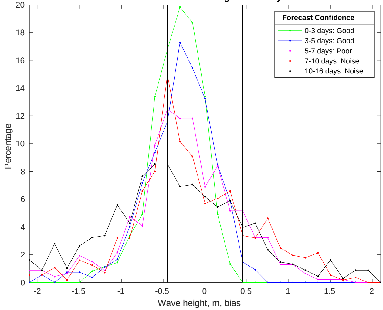
NDBC 46028 vs GFS Waves Bias Histogram: 07-May-2025
