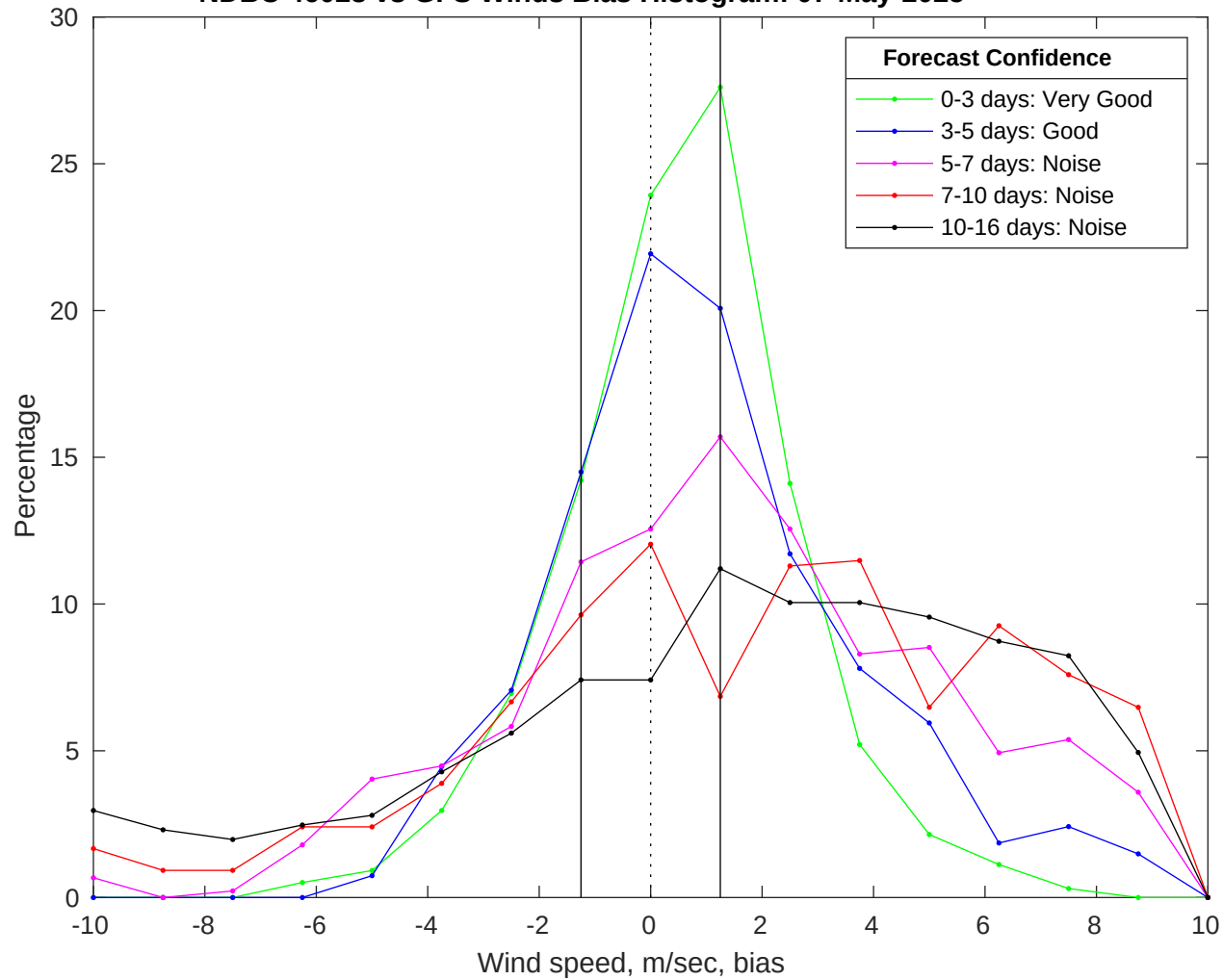
NDBC 46028 vs GFS Winds Bias Histogram: 07-May-2025
