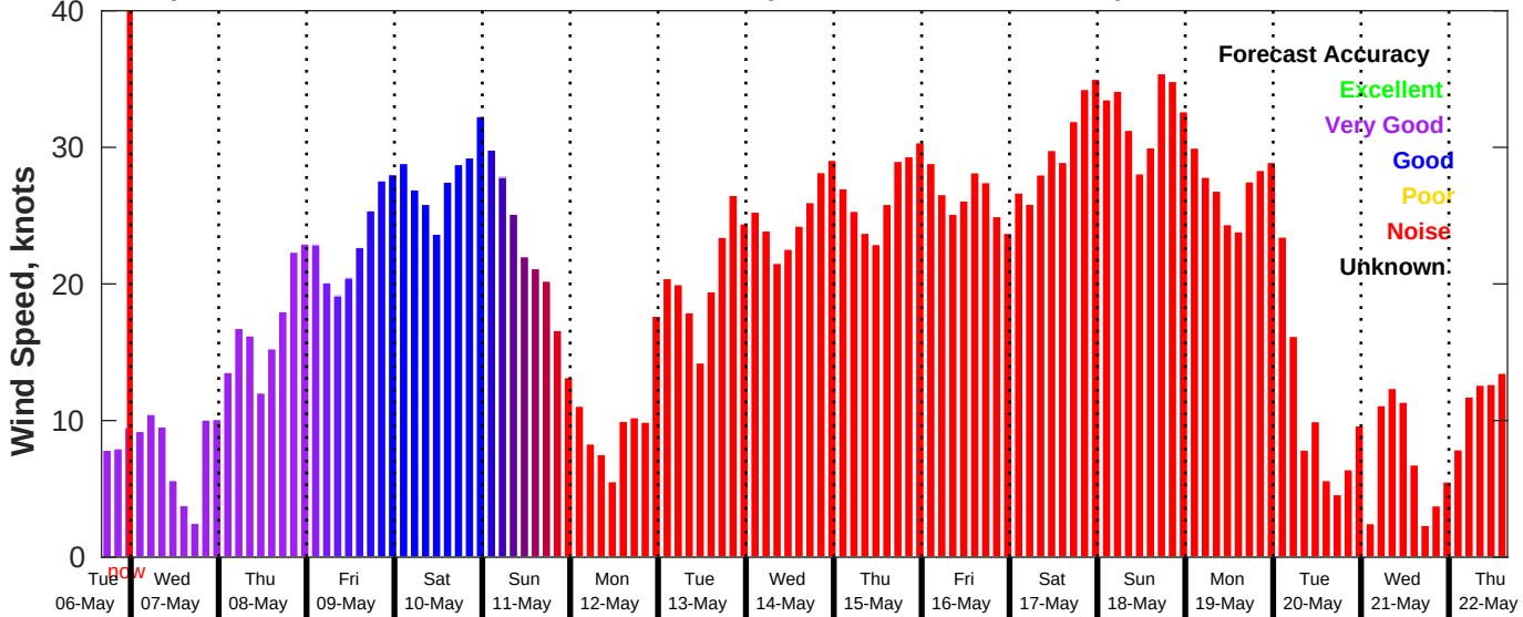
GFS Wind Speed Forecast for NDBC 46028 from 06-May-2025 16:00:00 to 22-May-2025 16:00:00
