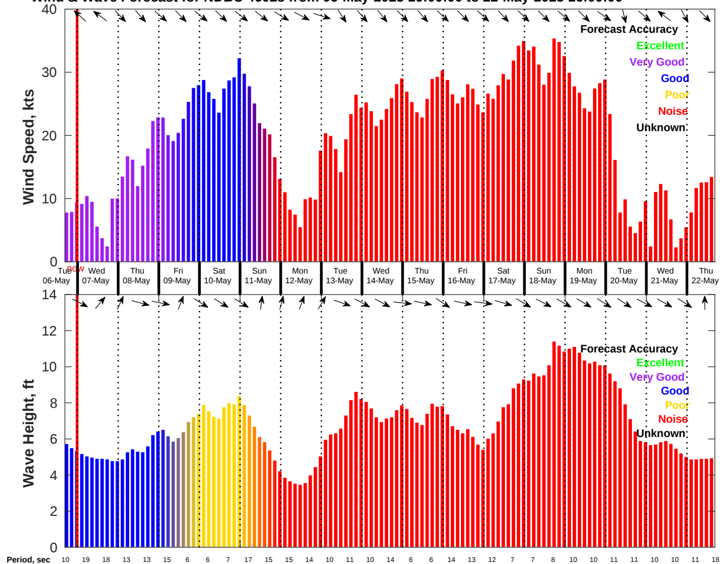
Wind & Wave Forecast for NDBC 46028 from 06-May-2025 16:00:00 to 22-May-2025 16:00:00
