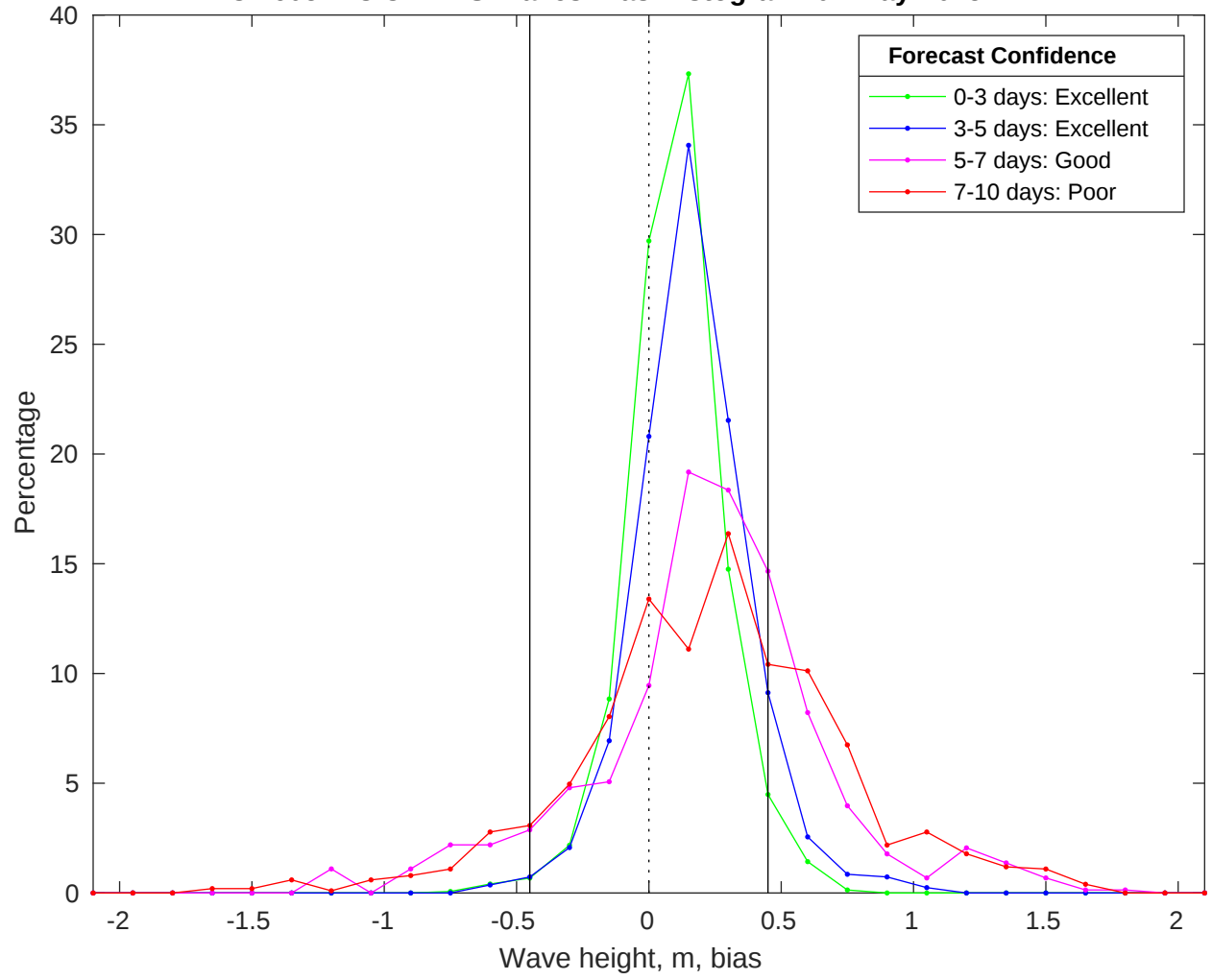
NDBC 46054 vs CMEMS Waves Bias Histogram: 07-May-2025
