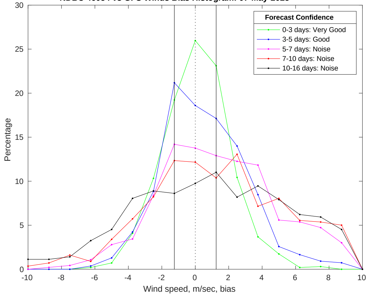
NDBC 46054 vs GFS Winds Bias Histogram: 07-May-2025
