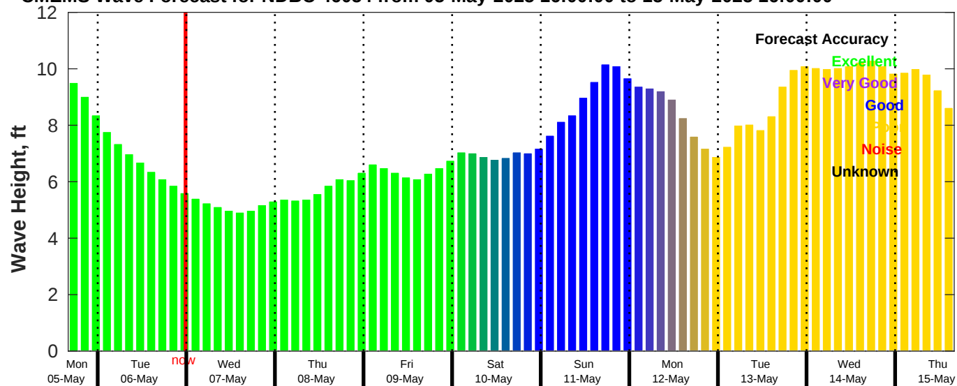
CMEMS Wave Forecast for NDBC 46054 from 05-May-2025 16:00:00 to 15-May-2025 16:00:00
