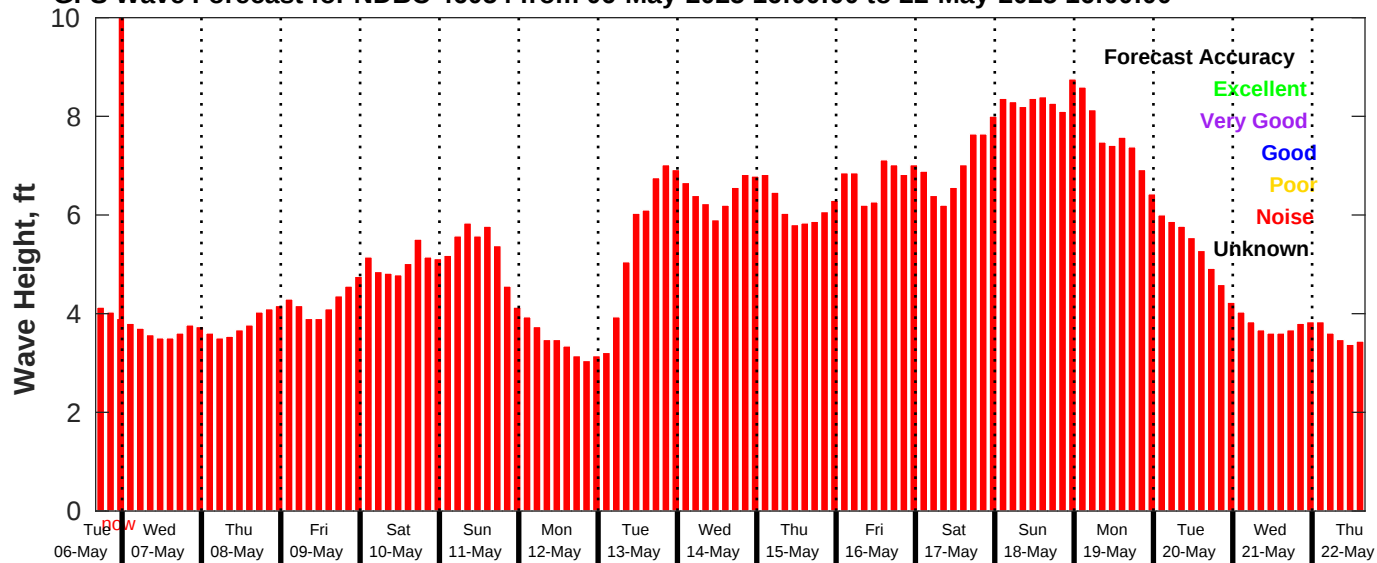
GFS Wave Forecast for NDBC 46054 from 06-May-2025 16:00:00 to 22-May-2025 16:00:00
