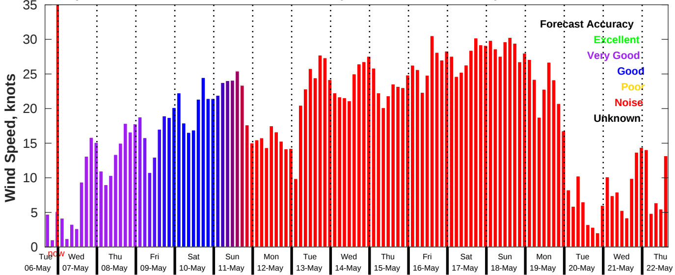
GFS Wind Speed Forecast for NDBC 46054 from 06-May-2025 16:00:00 to 22-May-2025 16:00:00
