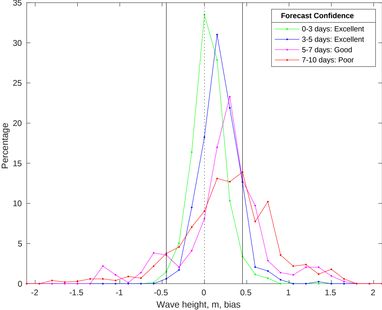
NDBC 46069 vs CMEMS Waves Bias Histogram: 07-May-2025
