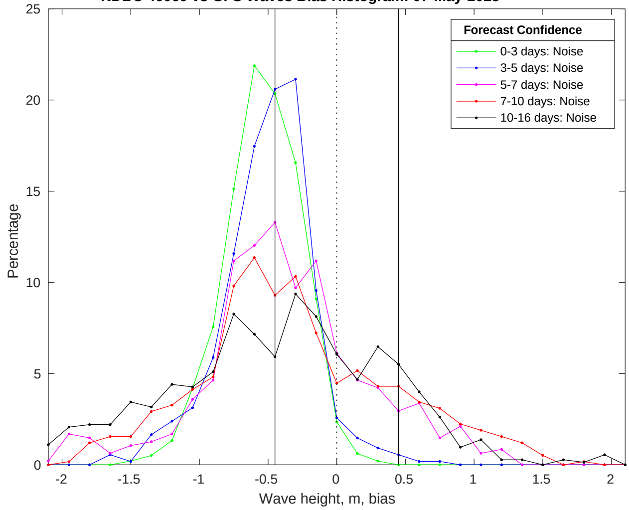
NDBC 46069 vs GFS Waves Bias Histogram: 07-May-2025
