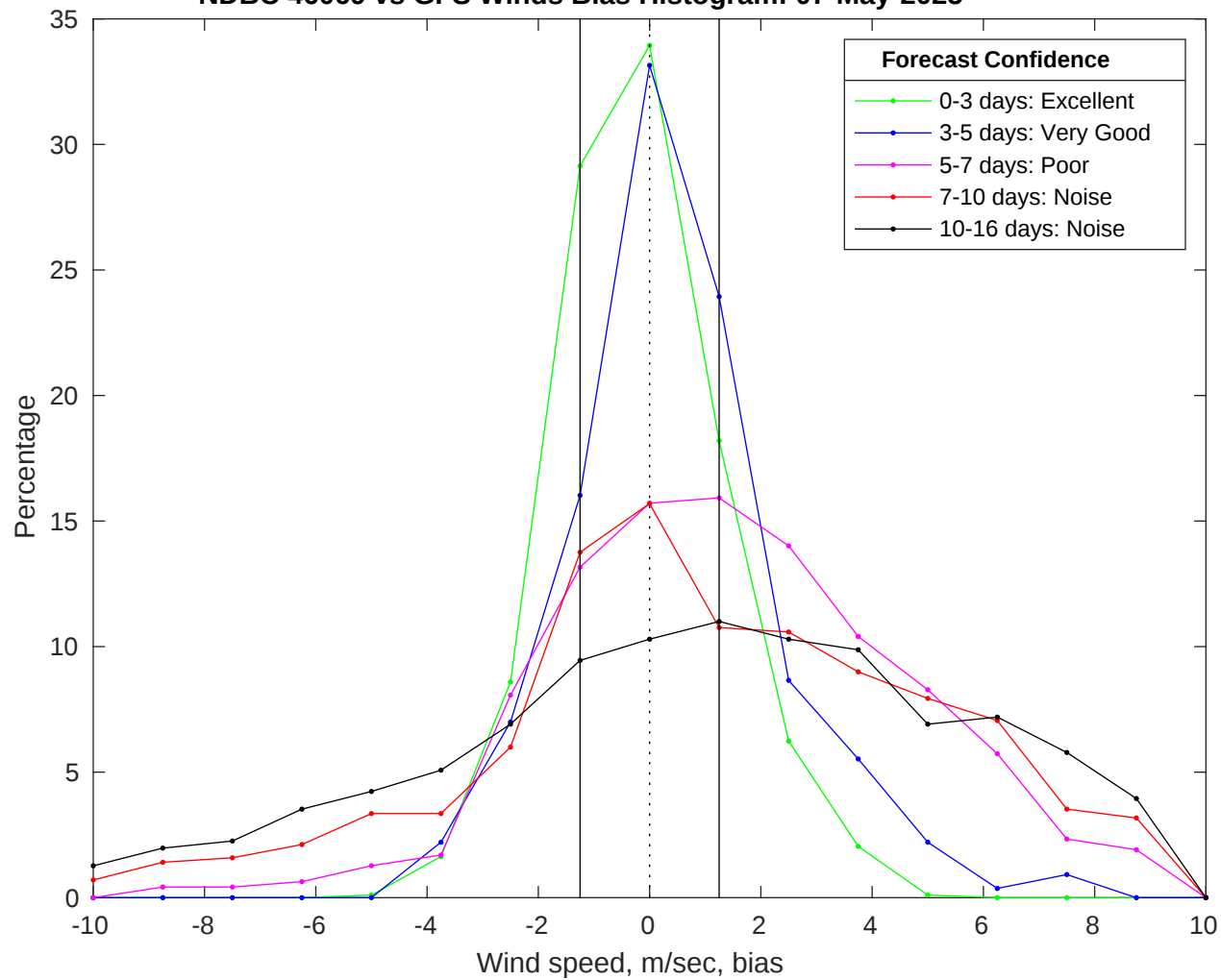
NDBC 46069 vs GFS Winds Bias Histogram: 07-May-2025
