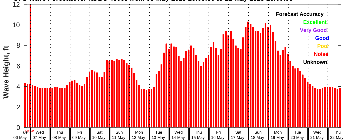
GFS Wave Forecast for NDBC 46069 from 06-May-2025 16:00:00 to 22-May-2025 16:00:00
