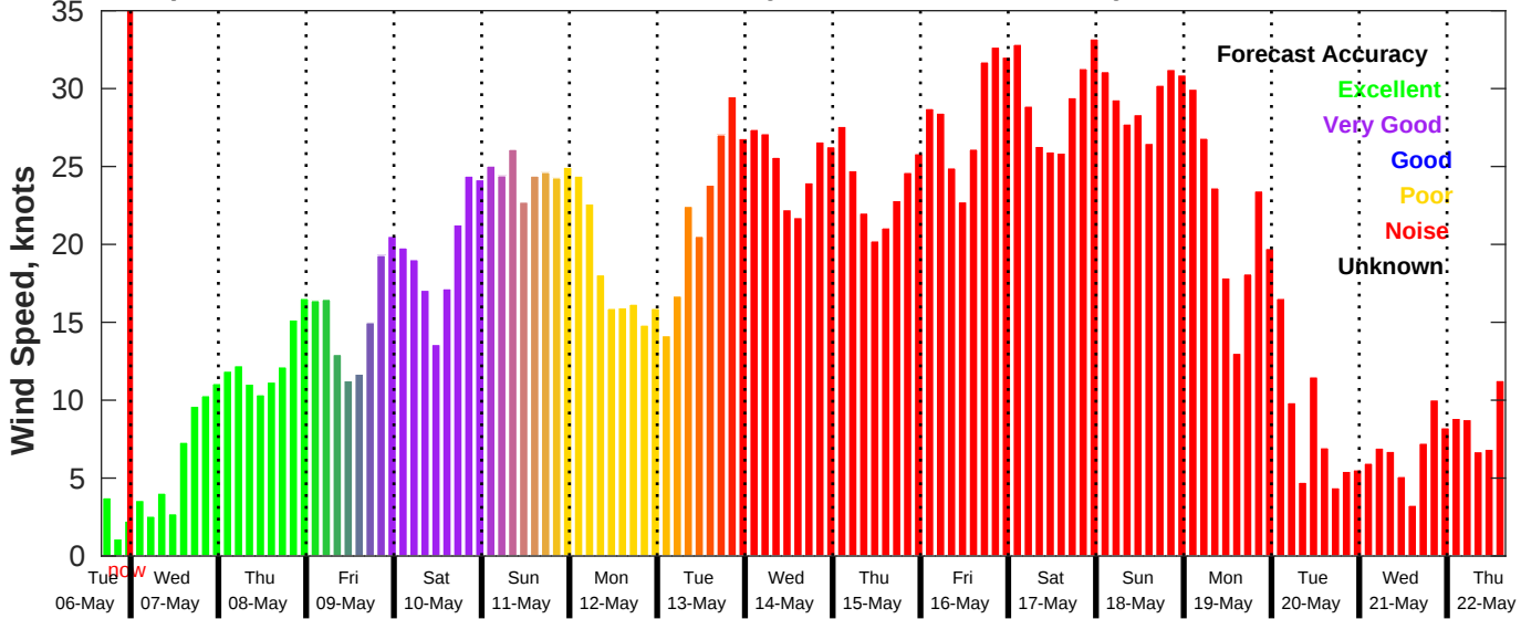
GFS Wind Speed Forecast for NDBC 46069 from 06-May-2025 16:00:00 to 22-May-2025 16:00:00
