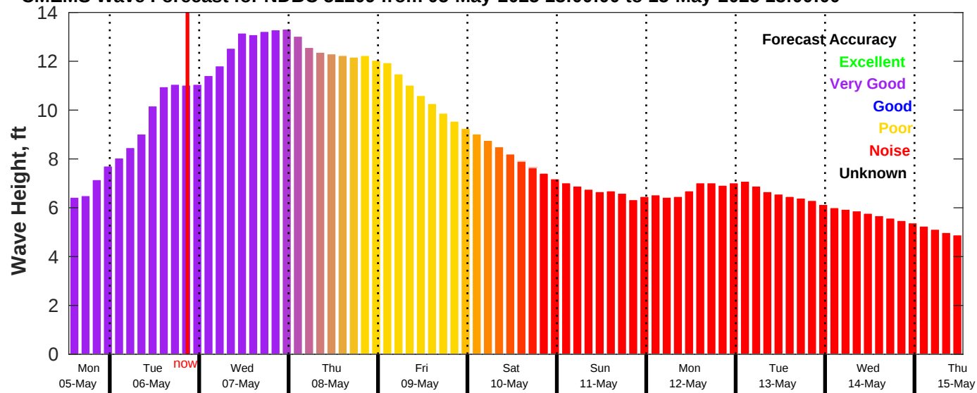
CMEMS Wave Forecast for NDBC 51209 from 05-May-2025 13:00:00 to 15-May-2025 13:00:00
