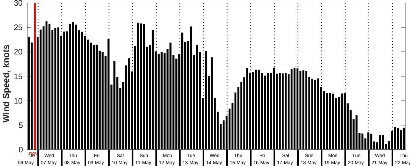
GFS Wind Speed Forecast for NDBC 51209 from 06-May-2025 13:00:00 to 22-May-2025 13:00:00
