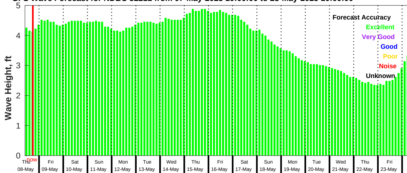
GFS Wave Forecast for NDBC 52211 from 07-May-2025 10:00:00 to 23-May-2025 10:00:00
