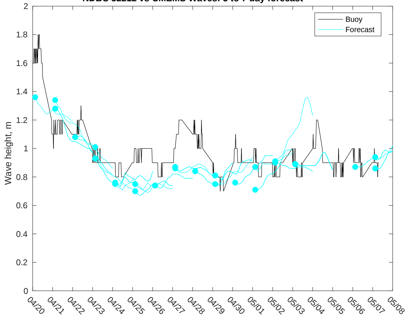
NDBC 52212 vs CMEMS Waves: 5 to 7 day forecast
